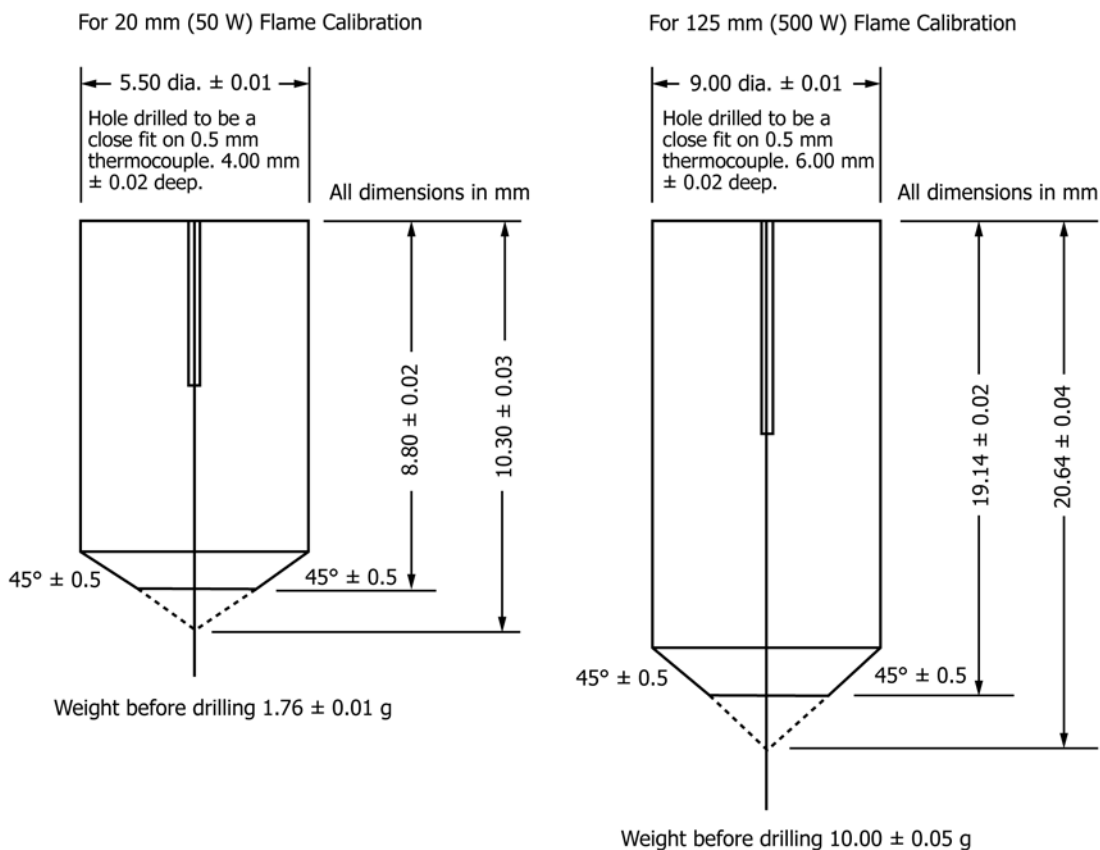
FIG. 1 Copper Slug for Thermal Sensor
